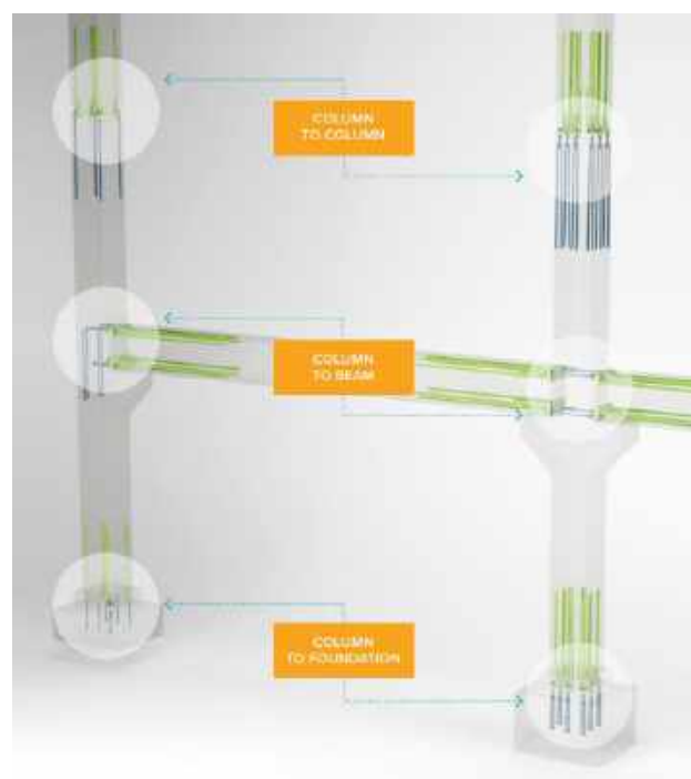
Figure 1. Variants of application of bolted connections
