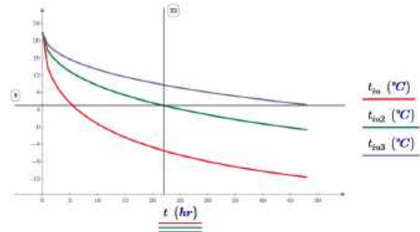
Figure 2. The change in internal air temperature when the heating system is turned off according to the dependence [4] with a variation in the linear dimensions of the internal load-bearing massive structures, t_{in} corresponds to 35 m 2 of wall (one partition 10 m long), t_{in2} - 70 m 2 of wall (two partitions 10 m long), t_{in3} - 105 m 2 of wall (three partitions 10 m long)
