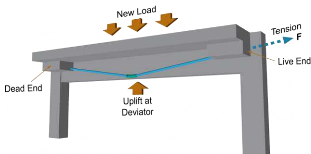
Figure 1. Schematic diagram of external reinforcement "External Post-Tensioning"
