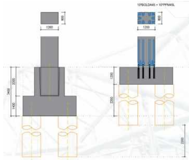
Figure 2. Options for connecting the foundation to the column that were considered.
