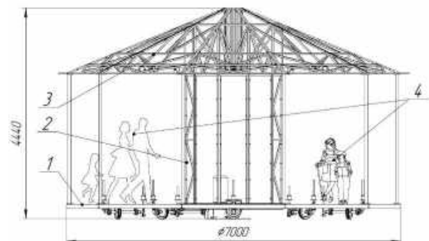
Figure 1. Construction of the carousel attraction with inclusive access
